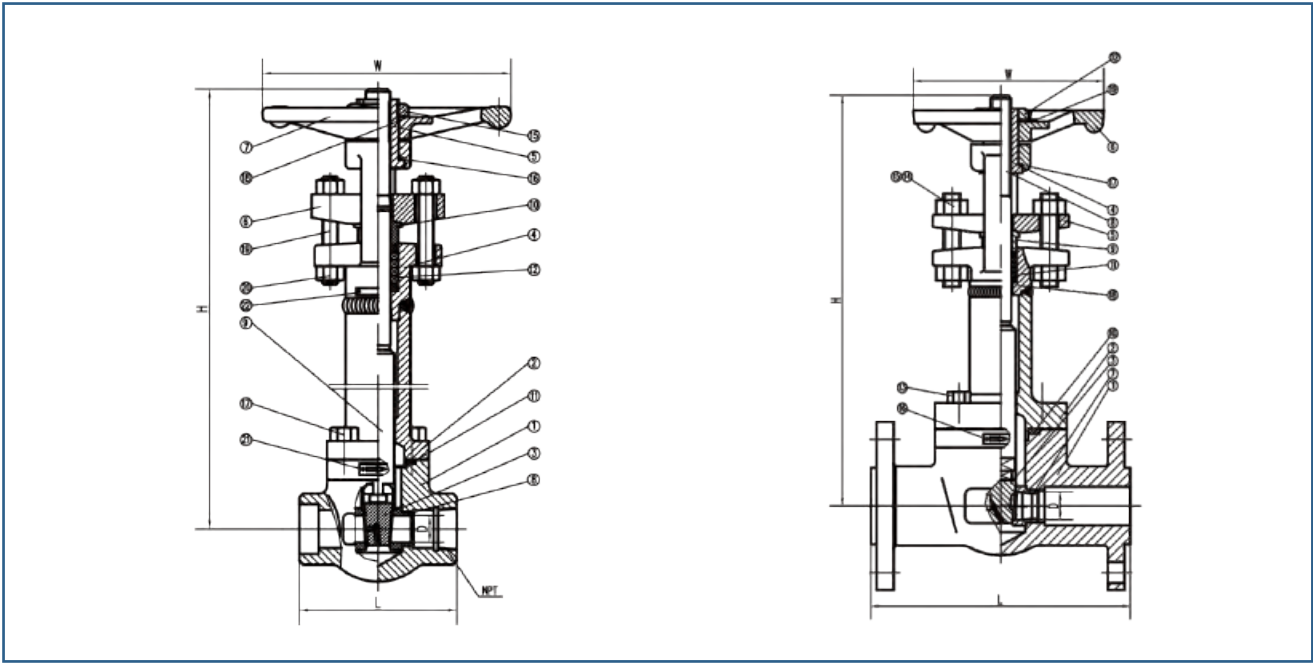
Bolted Bonnet
