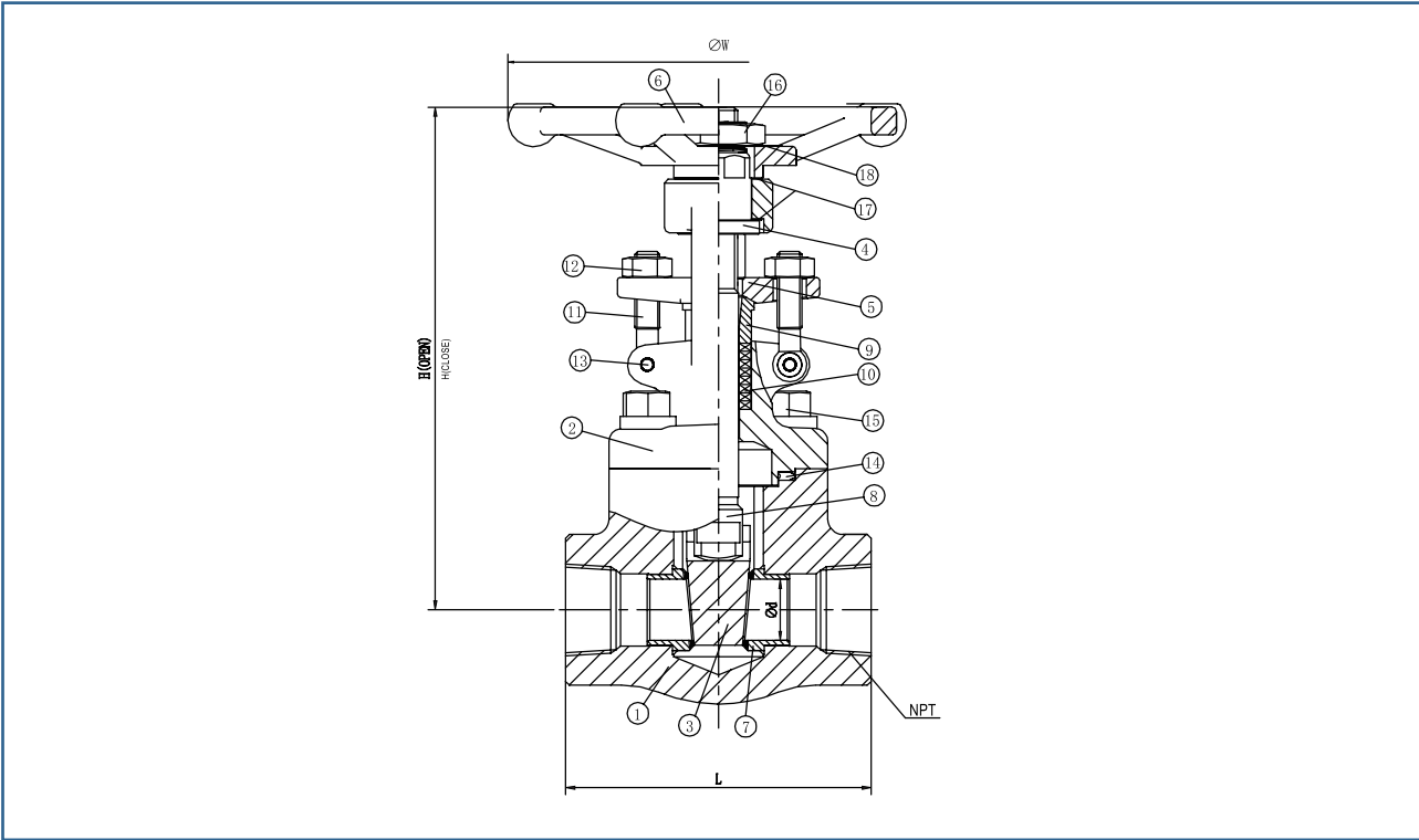
Bolted Bonnet
